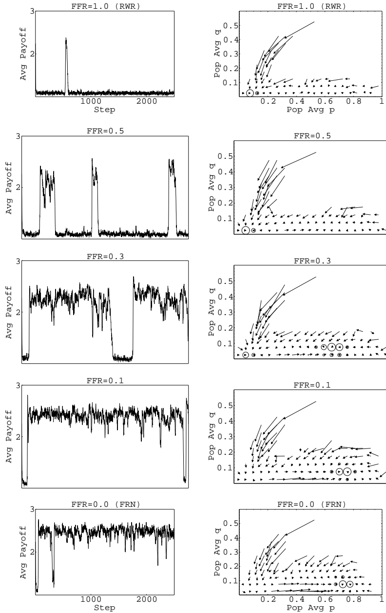
Figure 2: Average score per move (left column) for typical single runs, and p - q plots (right column) for a series of cases with decreasing (down the page) fraction of temporary random connections (RWR) added to fixed random connections (FRN). The p - q data is averaged over all 30 runs for each case.
