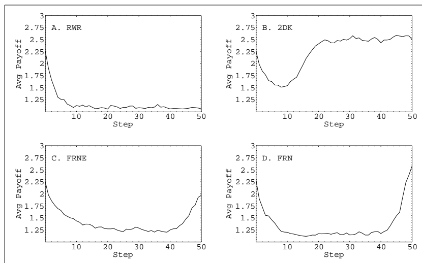
Figure 1: Average score per move over the initial fifty moves for four experimental conditions: RWR, 2DK, FRNE and FRN (see text for descriptions). The value for each period in each figure is the average score per move for all individuals in that period over all thirty histories (replications) for that condition.
